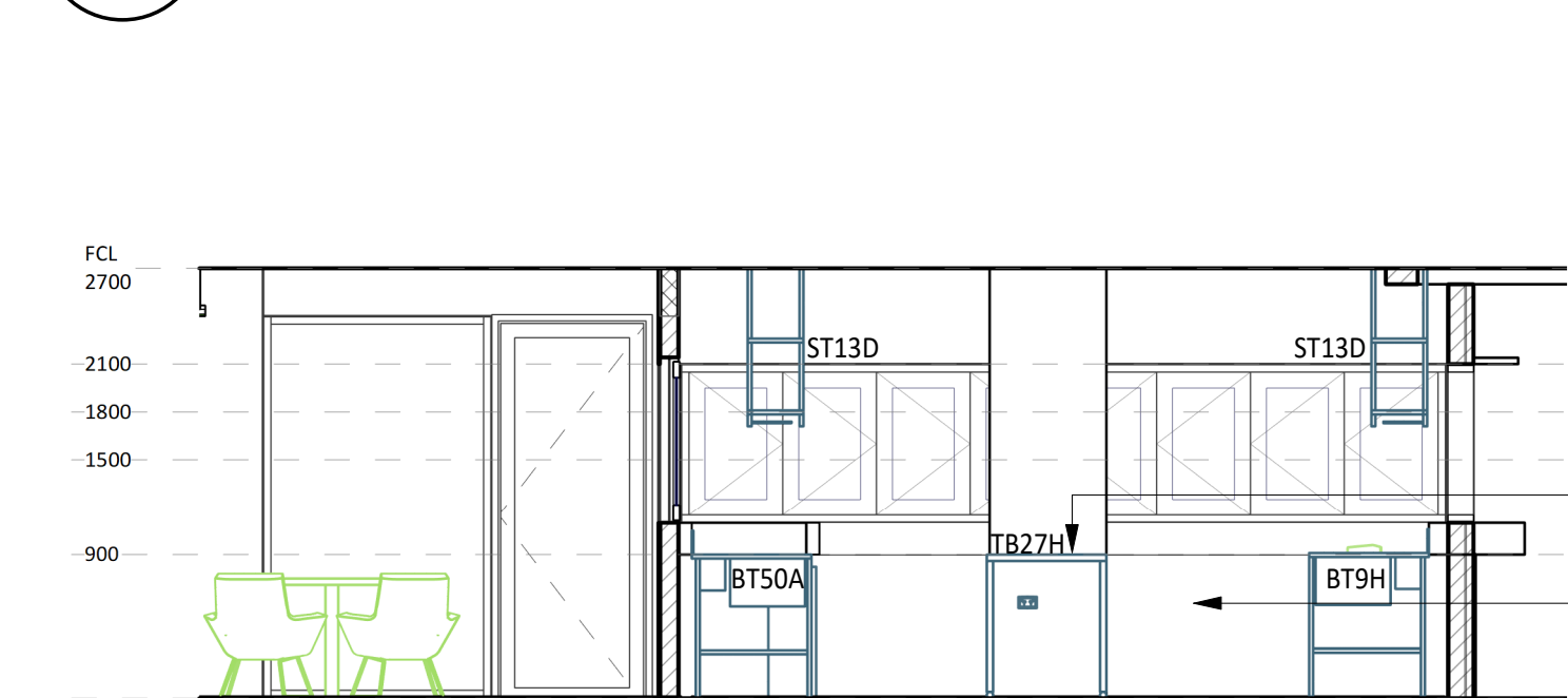
5 ELEVATION DETAIL 1 : 50
