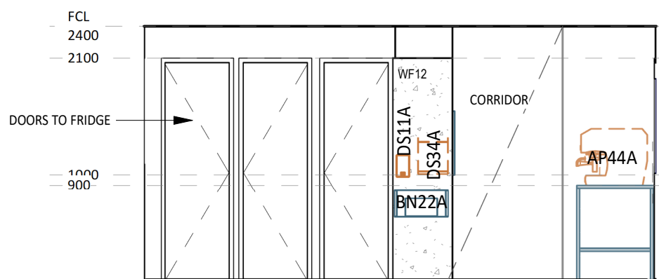
3 ELEVATION DETAIL 1 : 50
